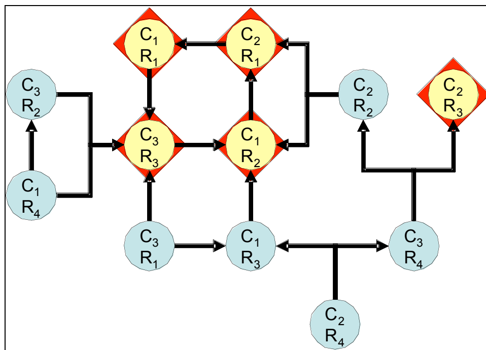
Figure 1: Example of configuration dominance.
